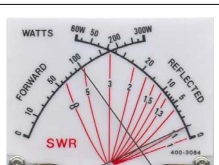
Figure 12. SWR/Wattmeter.
